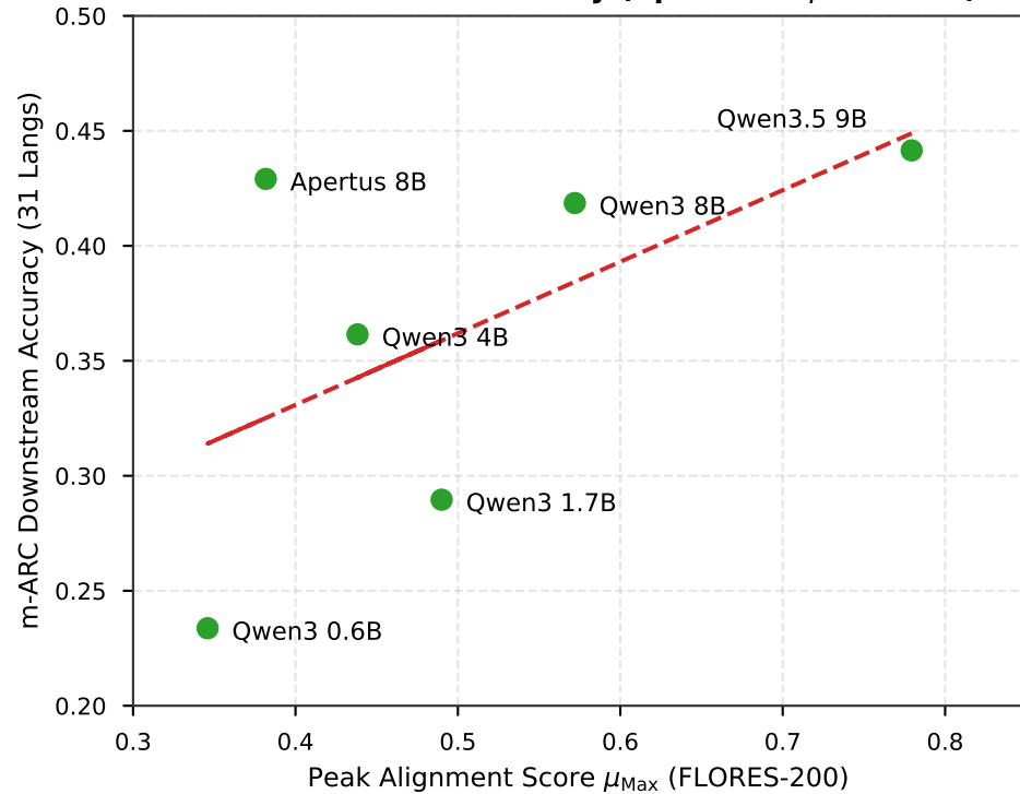
MEXA vs. m-ARC Accuracy (Spearman \rho = 0.600 )
