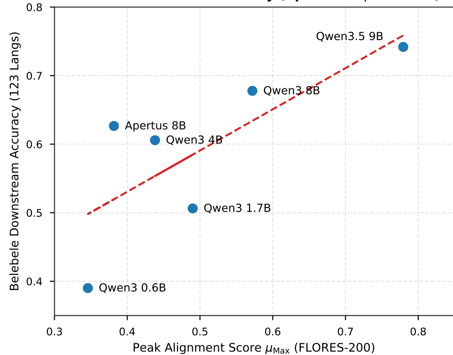
MEXA vs. Belebele Accuracy (Spearman \rho = 0.771 )
